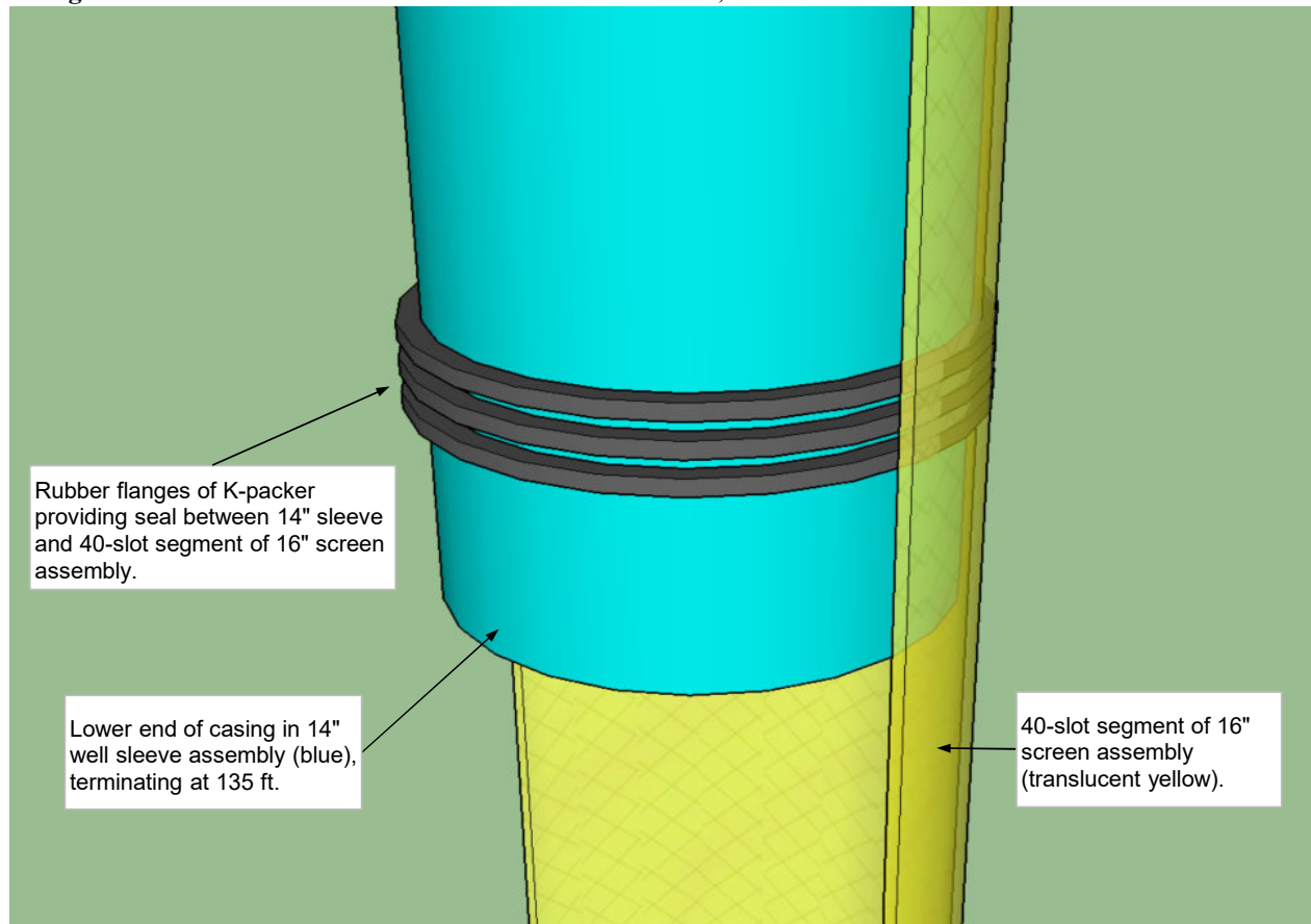
Figure 3 - Saranac Lake Well PW-1 Sleeve Insert - Detail, Lower Sleeve K-Packer
