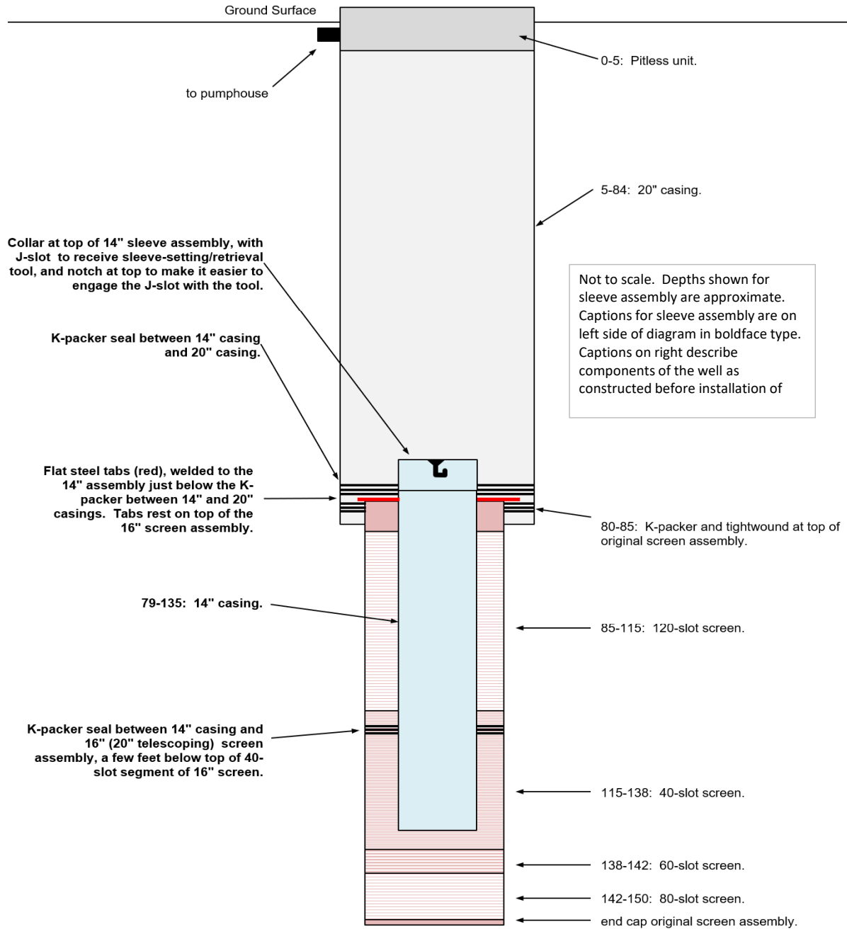
Figure 1 - Saranac Lake Well PW-1 Sleeve Insert Diagram
