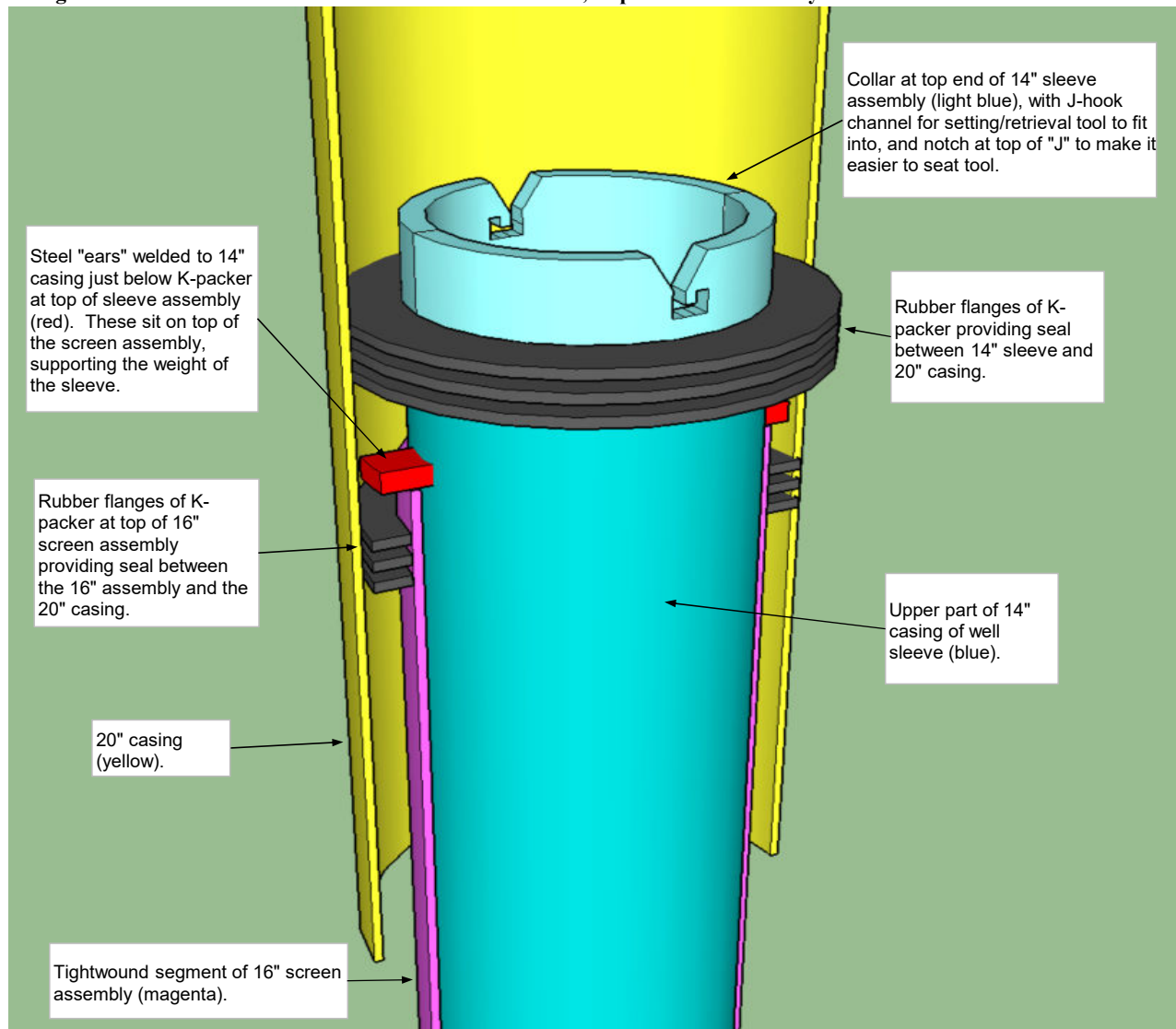
Figure 2 - Saranac Lake Well PW-1 Sleeve Insert - Detail, Top of Sleeve Assembly
